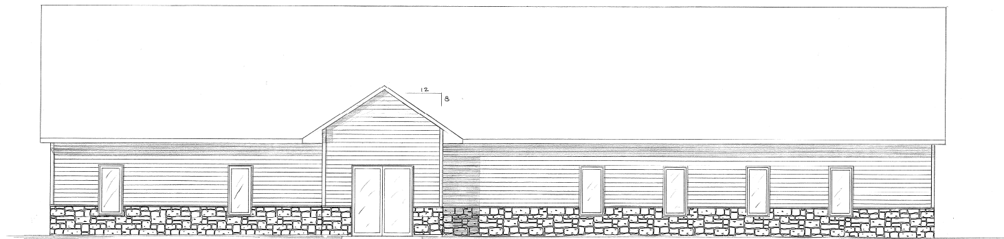
FRONT ELEVATION 1/4" = 1'-0"
